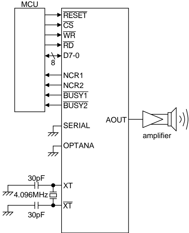
Parallel Interface
