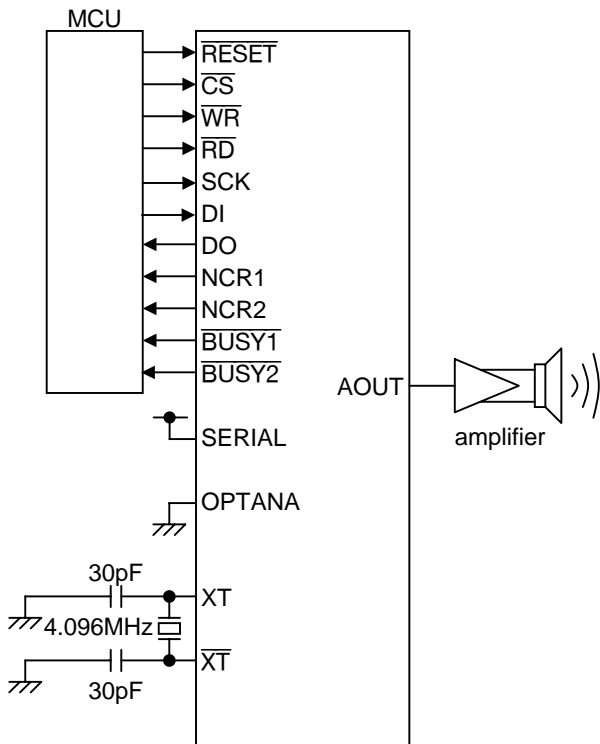
Serial Interface
