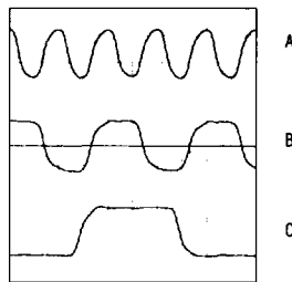
CLOCK/DATA (DIVIDE-BY-2 MODE)
