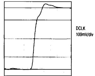
DIGITAL CLOCK (POSITIVE EDGE)
