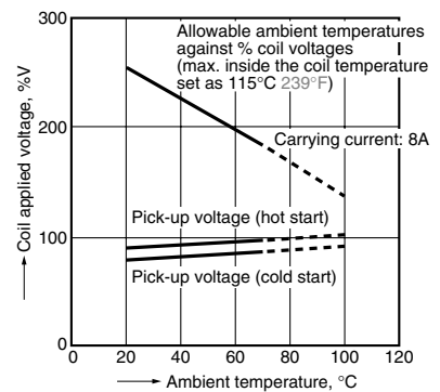
3. Ambient temperature characteristics and coil applied voltage
