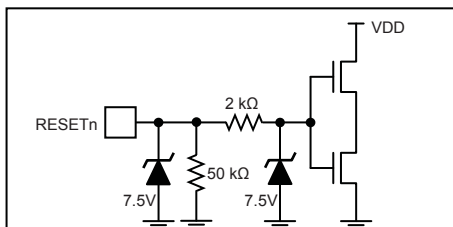
Figure 12e. RESETn Input
