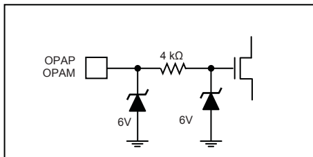
Figure 12h. Operational Amplifier Inputs
