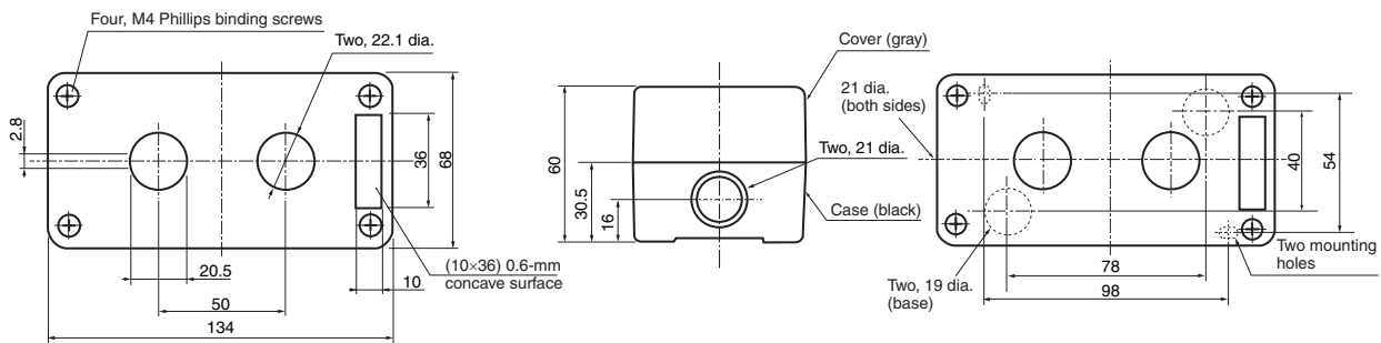
Cable Port Hole (Top View)
