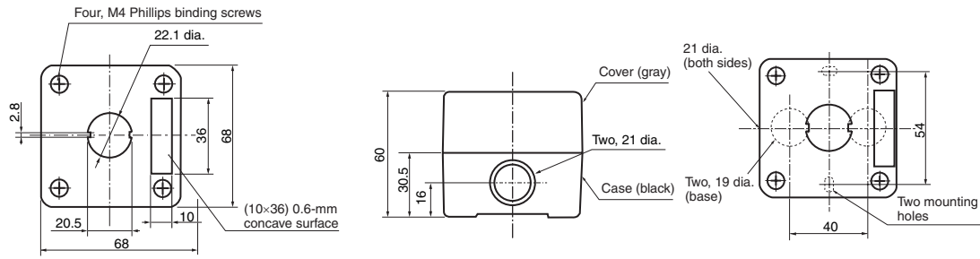
Cable Port Hole (Top View)
