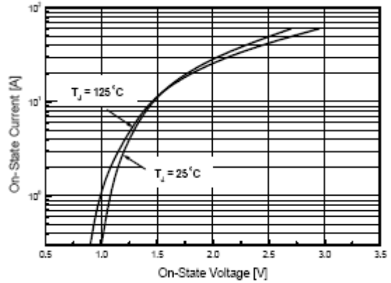
Fig.2 On-State Voltage
