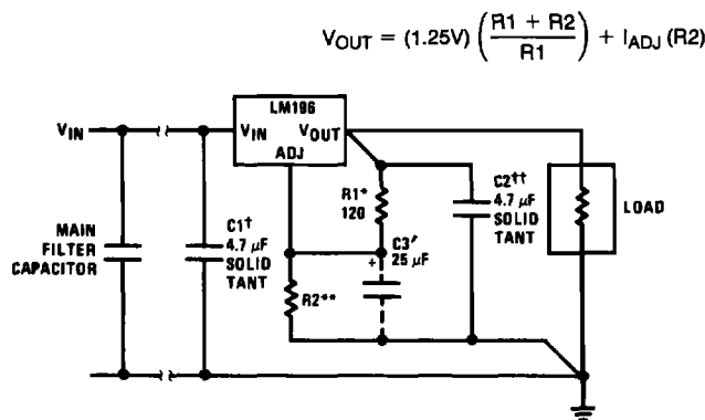
TL/H/9058-1 FIGURE 1. Basic 1.25V to 15V Regulator
