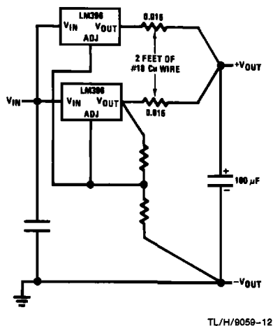
FIGURE 5a. Paralleling Regulators
