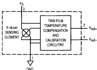
Figure 1. Temperature Compensated Pressure Sensor Schematic
