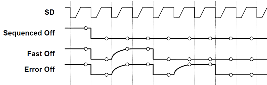
Figure 40. OK Severity Encoding Waveforms
