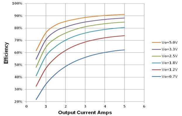
Figure 3. Efficiency vs. Load, V_{in} = 12 V, F_{sw} = 500 KHz
