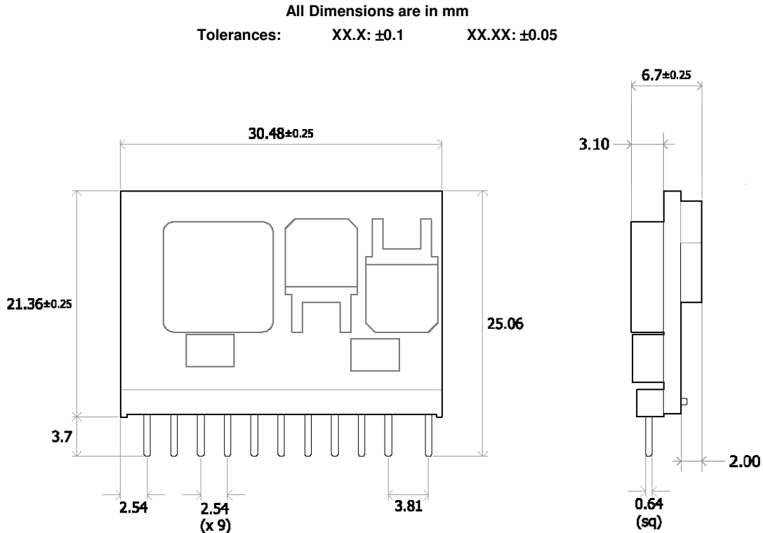
Figure 56. Mechanical Drawing
