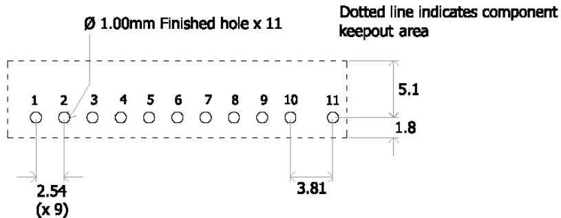
Figure 57. Recommended Footprint – Top View
