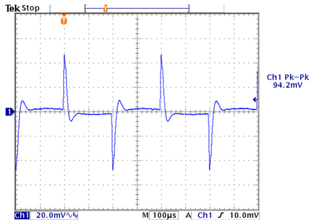
Figure 14 Transient Response with Regulation set to 0 mV/A.
