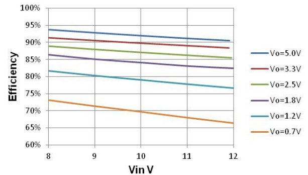
Figure 5. Efficiency vs Input Voltage at I_{out} = 5 A, F_{sw} = 500 KHz
