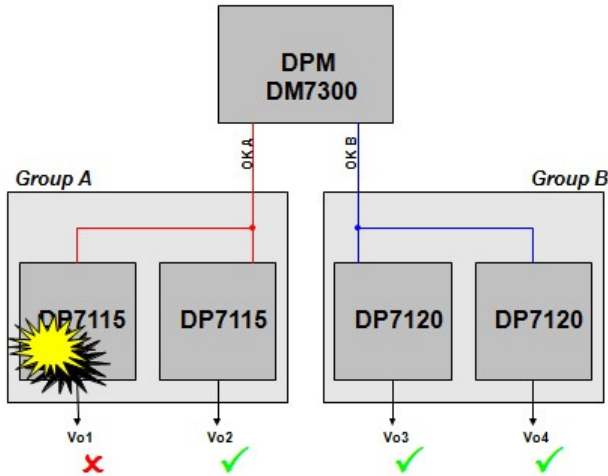
Figure 36. No Group Fault Propagation
