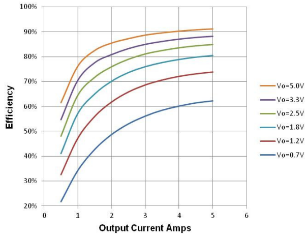
Figure 6. Efficiency vs Load, Vin=12V, Fsw=1MHz
