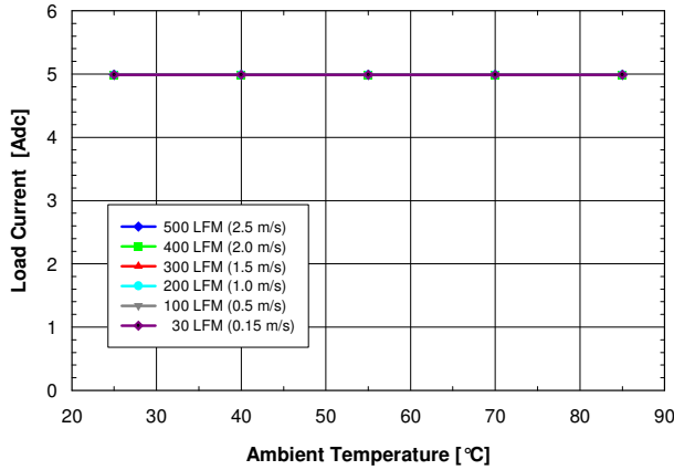
Figure 1. Available output current vs. ambient air temperature and airflow rates for converter DP8105 mounted horizontally with air flowing from input to output, MOSFET temperature \leq 120 °C, V_{in} = 12 V, V_{out} = 5 V, and F_{sw} = 500 KHz
