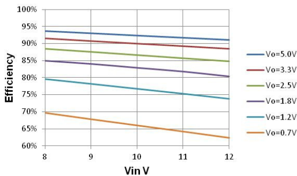
Figure 8. Efficiency vs Input Voltage at Iout=5A, Fsw=1MHz
