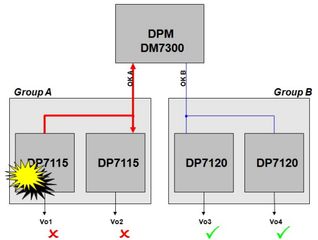
Figure 38. Intra Group Fault Propagation
