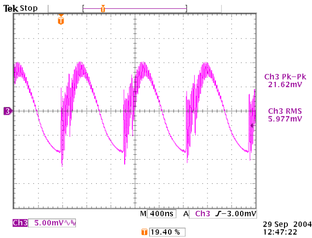
Figure 45. Output Voltage Noise, Full Load, No Interleave
