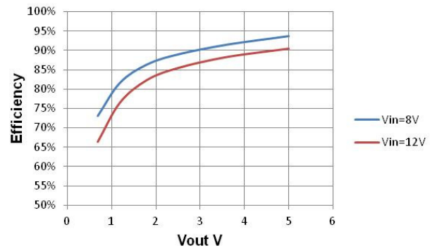
Figure 4. Efficiency vs. Output Voltage, I_{out} = 5 A, F_{sw} = 500 kHz
