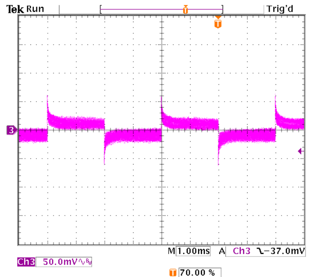
Figure 49. Transient Response with Regulation set to 6.53 mV/A
