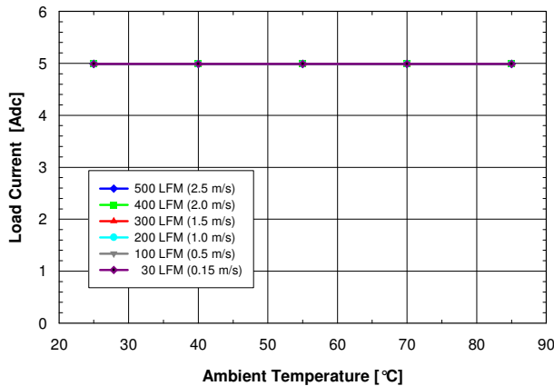
Figure 2. Available output current vs. ambient air temperature and airflow rates for converter DP8105 mounted horizontally with air flowing from input to output, MOSFET temperature \leq 120 °C, V_{in} = 12 V, V_{out} = 5 V, and F_{sw} = 1 MHz
