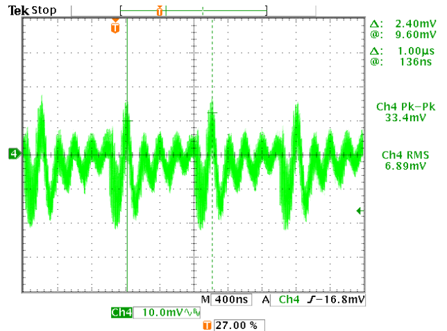
Figure 44. Input Voltage Noise with Interleave
