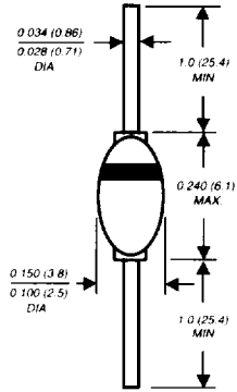
DO-204AP
