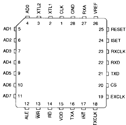
28-Pin PLCC
