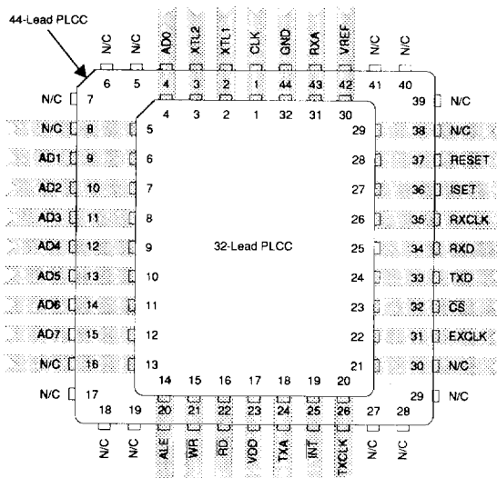
32, 44-Pin PLCC
