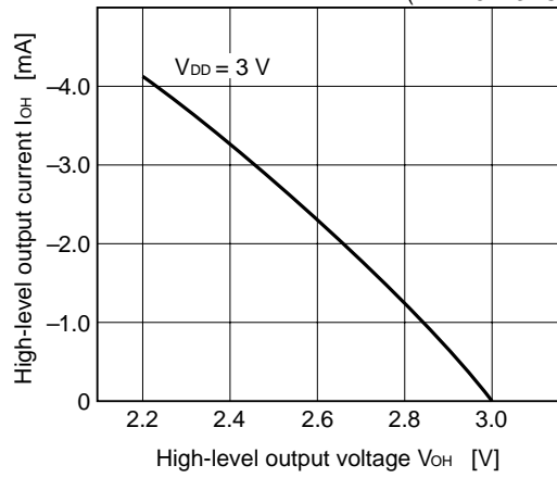
I_{OH} vs V_{OH} characteristic examples ( K_{VO} , I/O)
