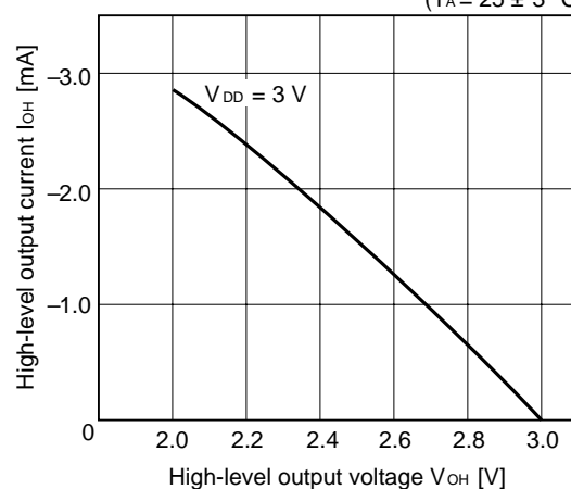
I_{OH} vs V_{OH} characteristic examples (S-OUT)
