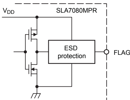
Figure 10. FLAG pin equivalent circuit
