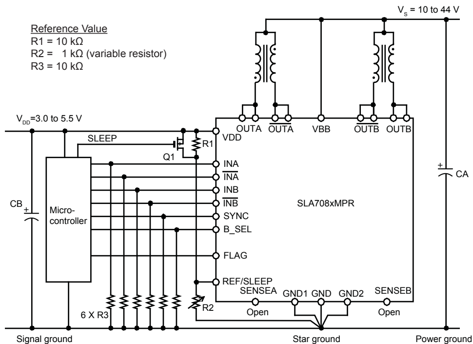
Figure 12. Typical application circuit using SLA7080MPR
