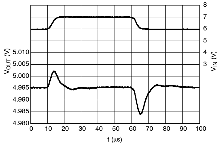
Figure 28. Line Transients, 5.0 V Version, t_R = t_F = 5 \mu s , I_{OUT} = 30 \text{ mA}
