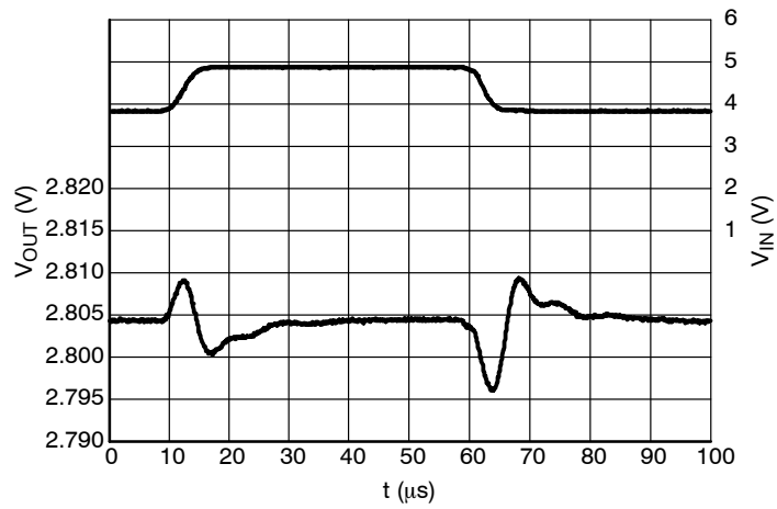
Figure 27. Line Transients, 2.8 V Version, t_R = t_F = 5 \mu s , I_{OUT} = 30 \text{ mA}
