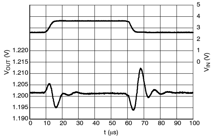
Figure 26. Line Transients, 1.2 V Version, t_R = t_F = 5 \mu s , I_{OUT} = 30 \text{ mA}
