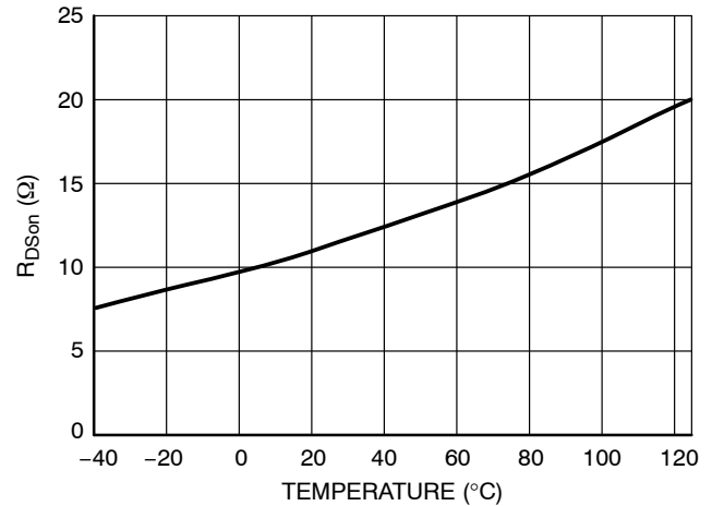
Figure 11. ON Resistance vs. Temperature
