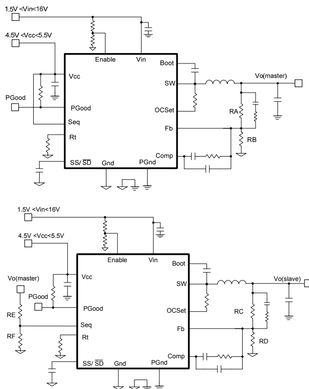
Fig. 8b. Application Circuit for Simultaneous Sequencing
