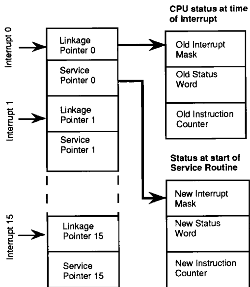
Figure 11: Interrupt Vectoring
