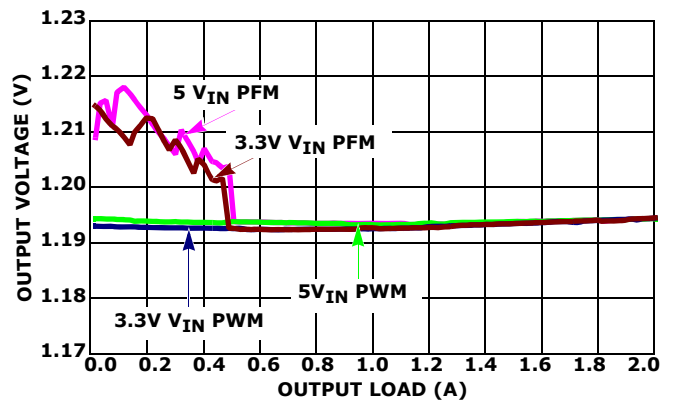
FIGURE 7. V OUT REGULATION vs LOAD, 2.25MHz, 1.2V, CHANNEL 1
