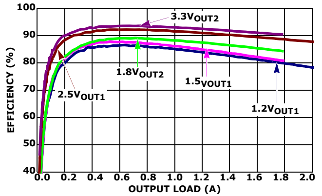
FIGURE 3. EFFICIENCY vs LOAD, 2.25MHz, 5V IN PWM
