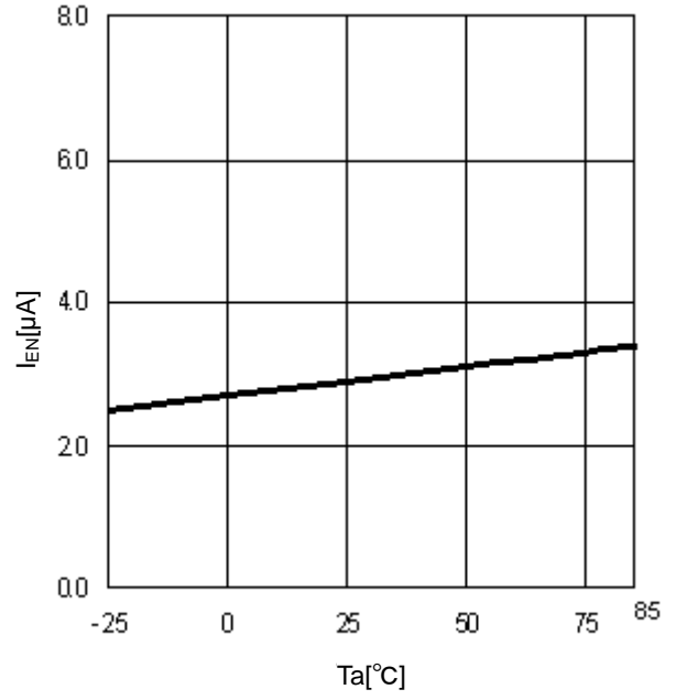
Figure 12. T_a - I_{EN}
