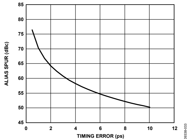
Figure 31. AS_{\text{TIMING}} as a Function of Timing Error
