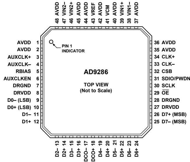
Figure 6. Pin Configuration
