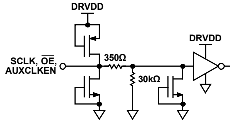
Figure 21. SCLK, OE, AUXCLKEN
