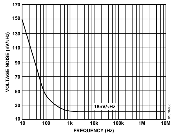
Figure 30. AD8115 Voltage Noise vs. Frequency
