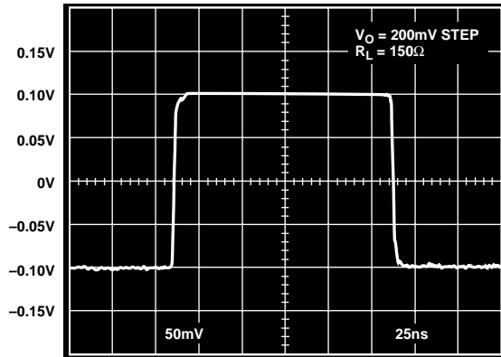
Figure 31. AD8114 Pulse Response, Small Signal
