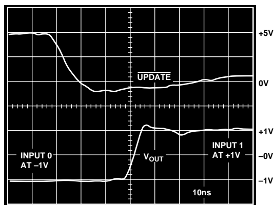
Figure 33. AD8114 Switching Time
