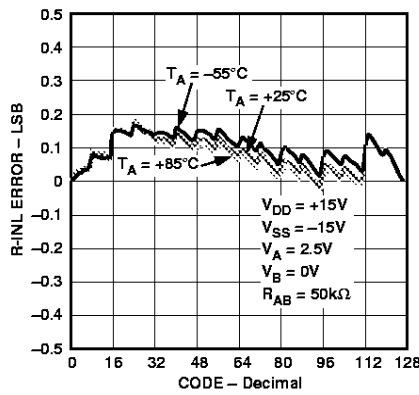
Figure 3. Resistance Step Position Nonlinearity Error vs. Code
