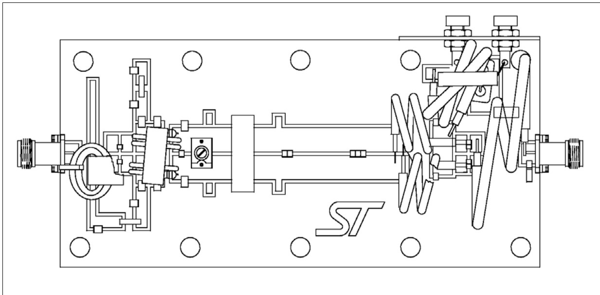
Figure 11. Circuit layout
