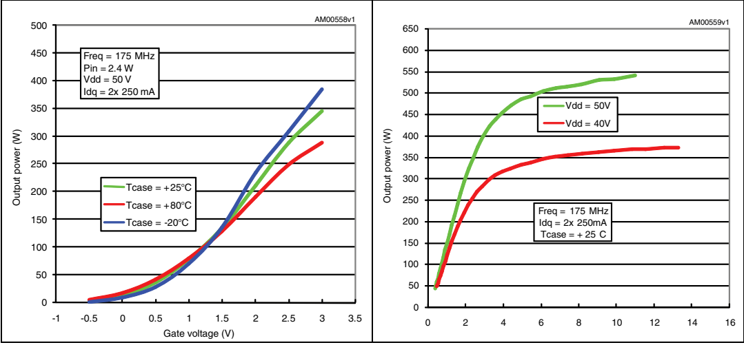
Figure 5. Output power vs gate voltage Figure 6. Output power vs input power
