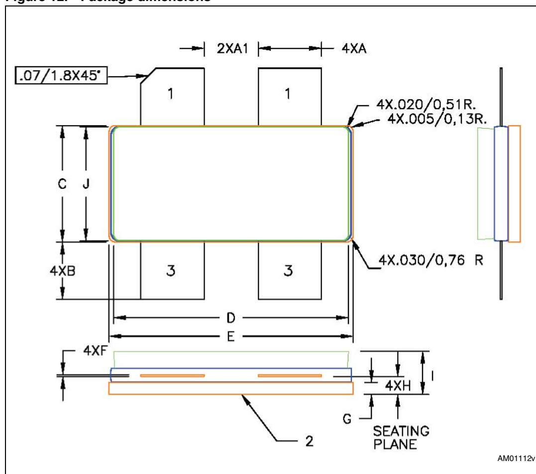
Figure 12. Package dimensions
