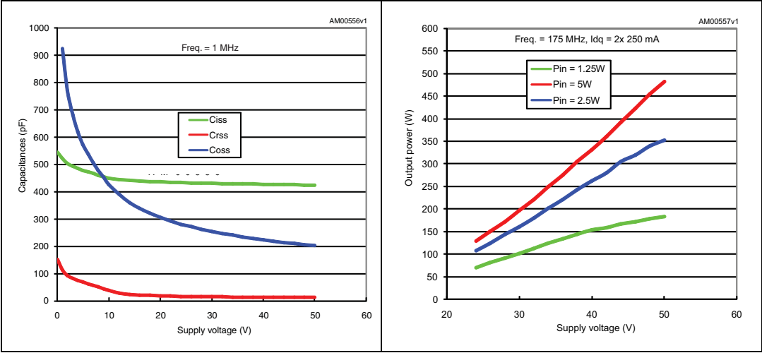
Figure 3. Capacitances vs drain supply voltage Figure 4. Output power vs drain supply voltage
