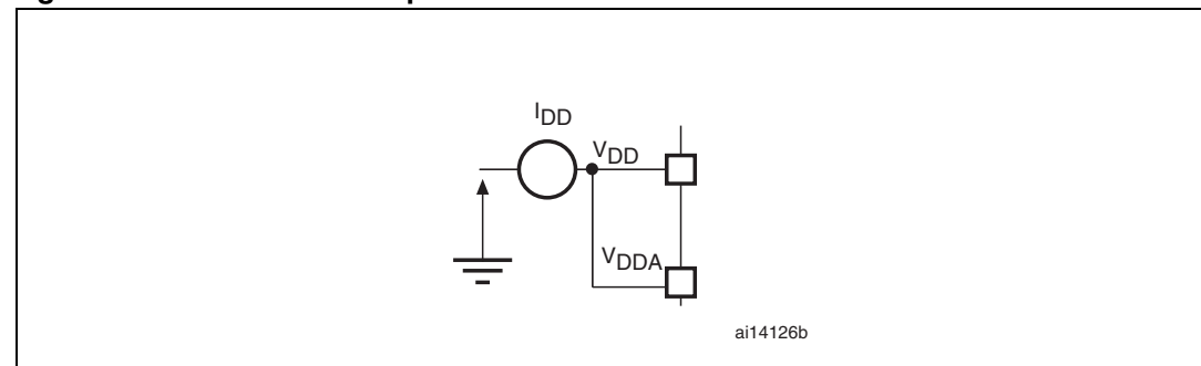
Figure 16. Current consumption measurement scheme
