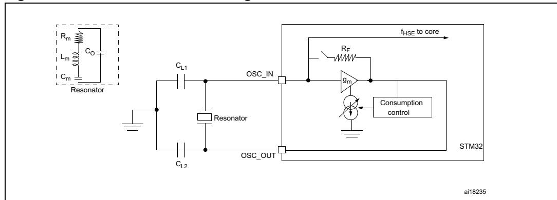
Figure 19. HSE oscillator circuit diagram
