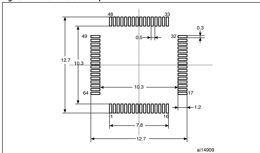
Figure 41. Recommended footprint
