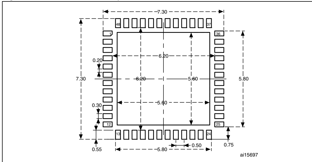
Figure 45. Recommended footprint
