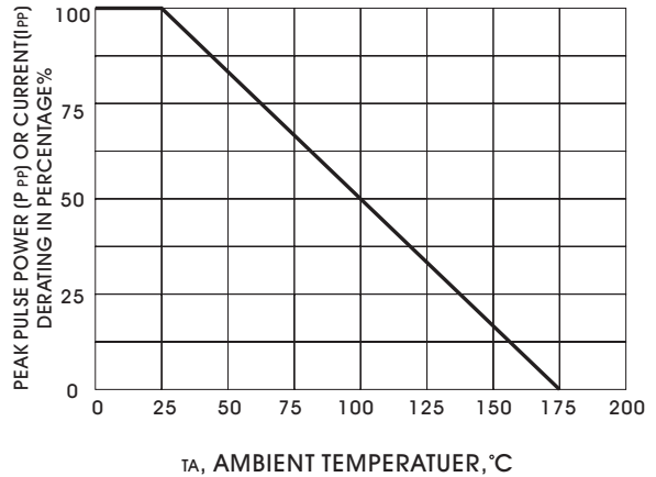
FIGURE 2-PULSE DERATING CURVE
