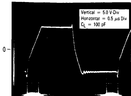
FIGURE 25 — LARGE-SIGNAL
