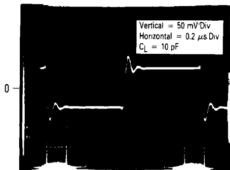
FIGURE 26 — SMALL-SIGNAL
