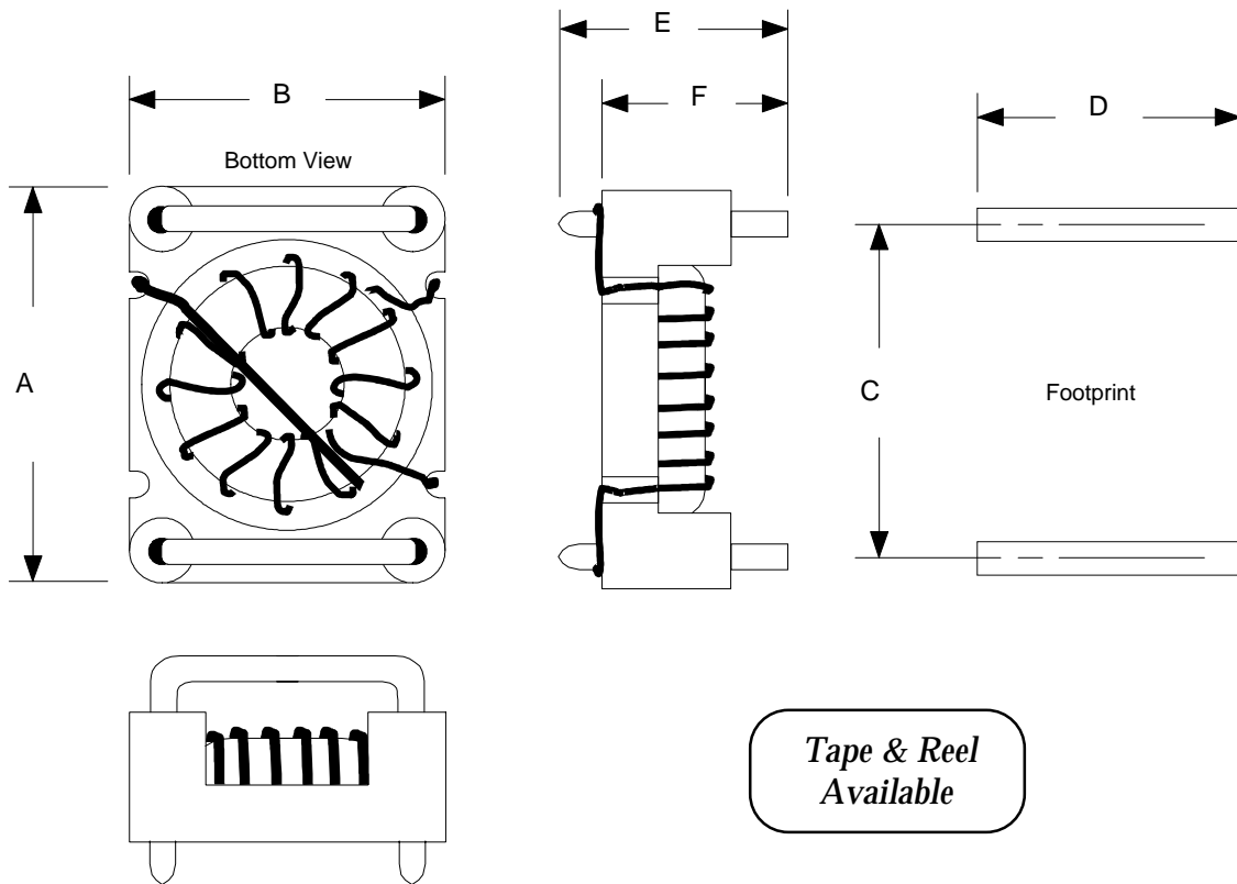
Package Dimensions in Inches
