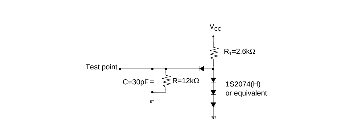
Figure 83 Timing Load Circuit
