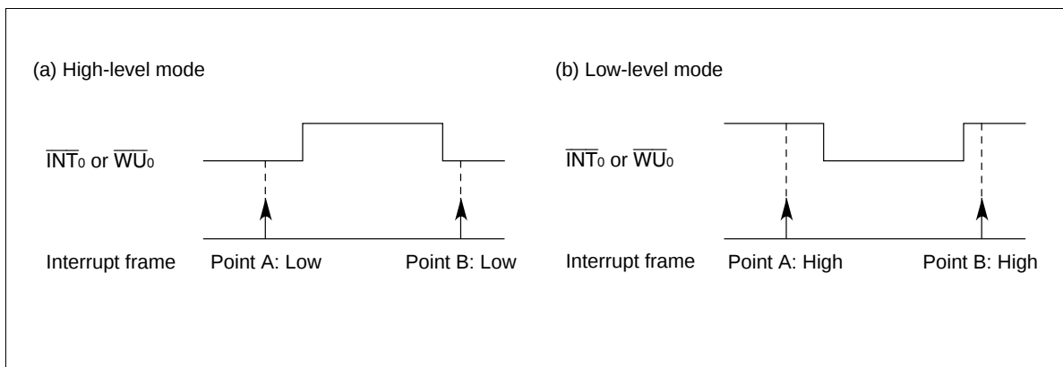
Figure 19 Sampling Examples
