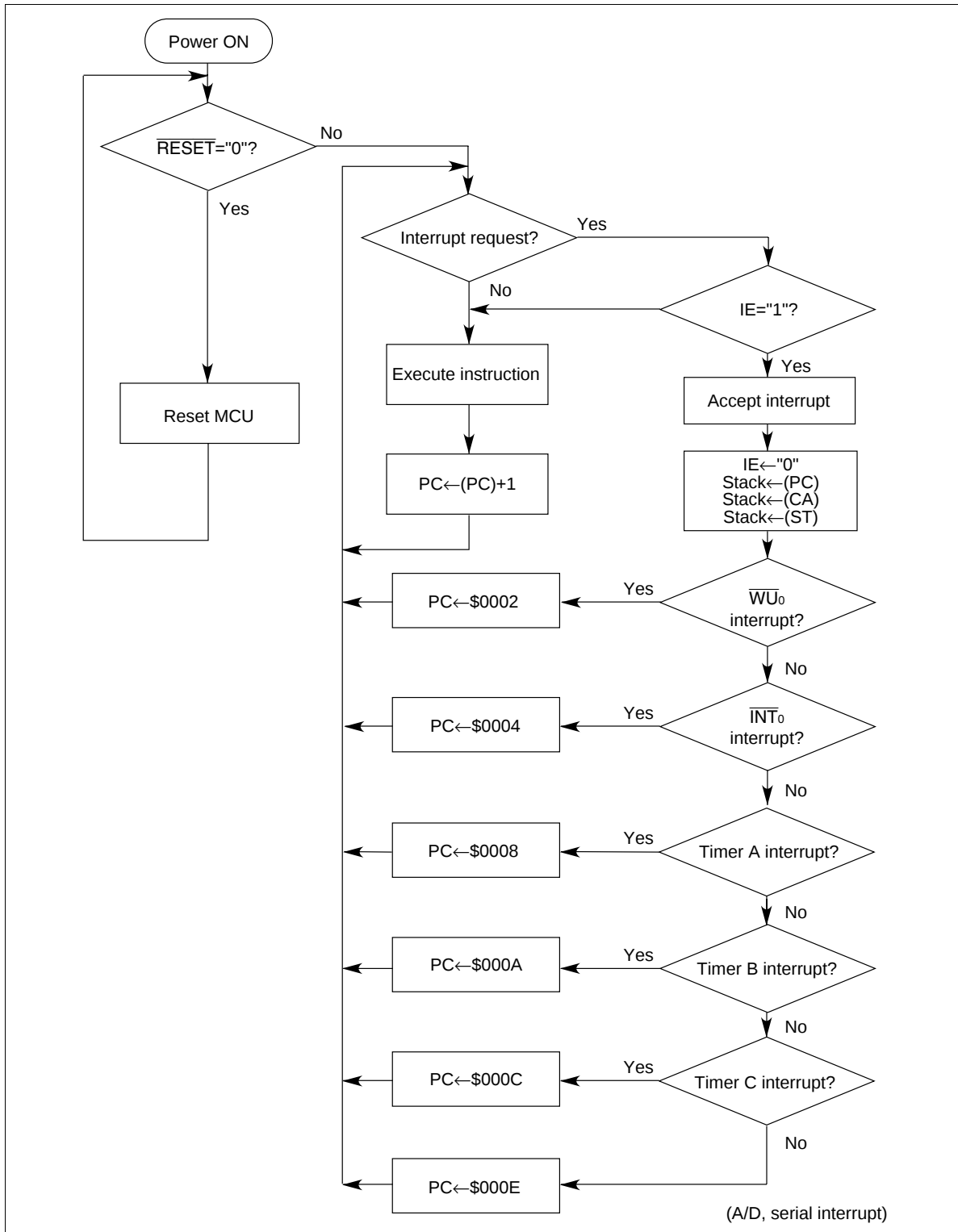
Figure 10 Interrupt Handling Flowchart
