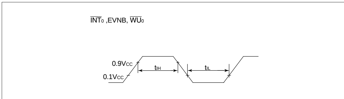
Figure 80 Interrupt Timing
