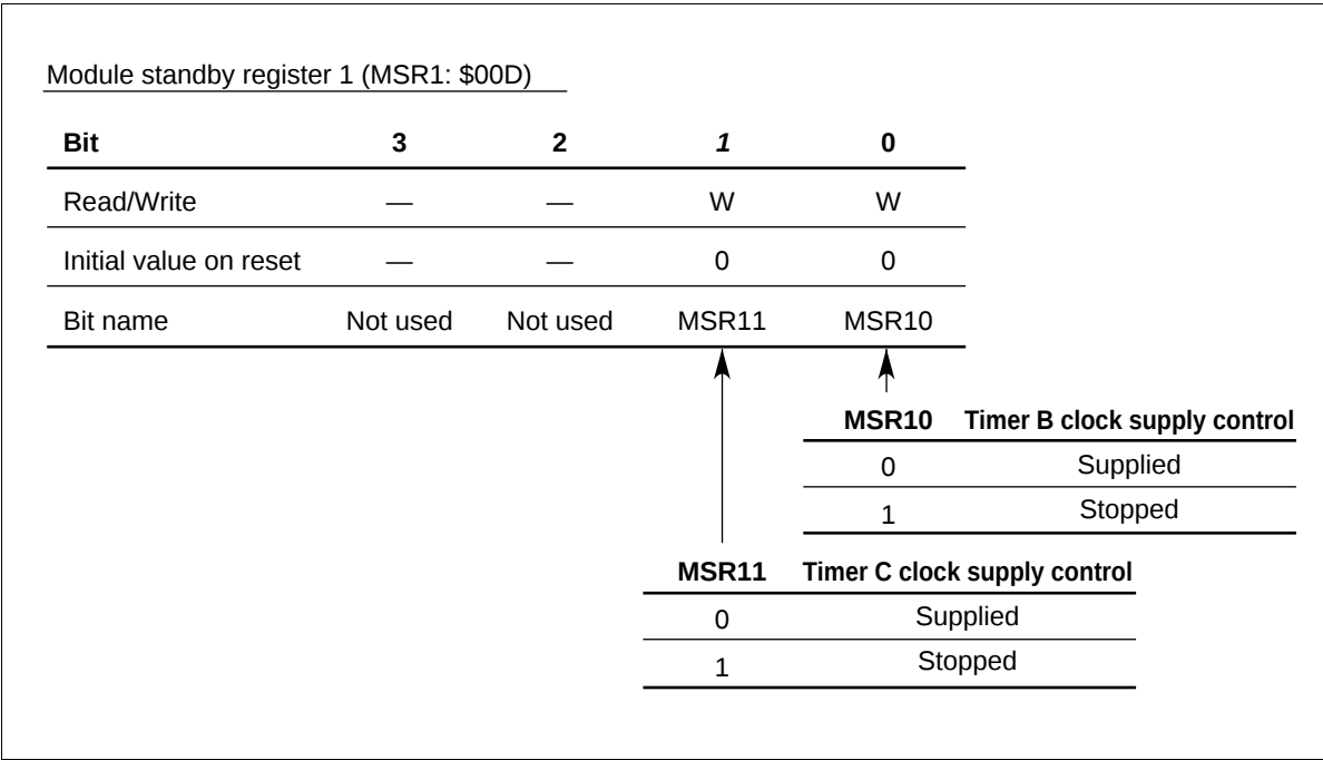
Figure 43 Module Standby Register 1 (MSR1)
