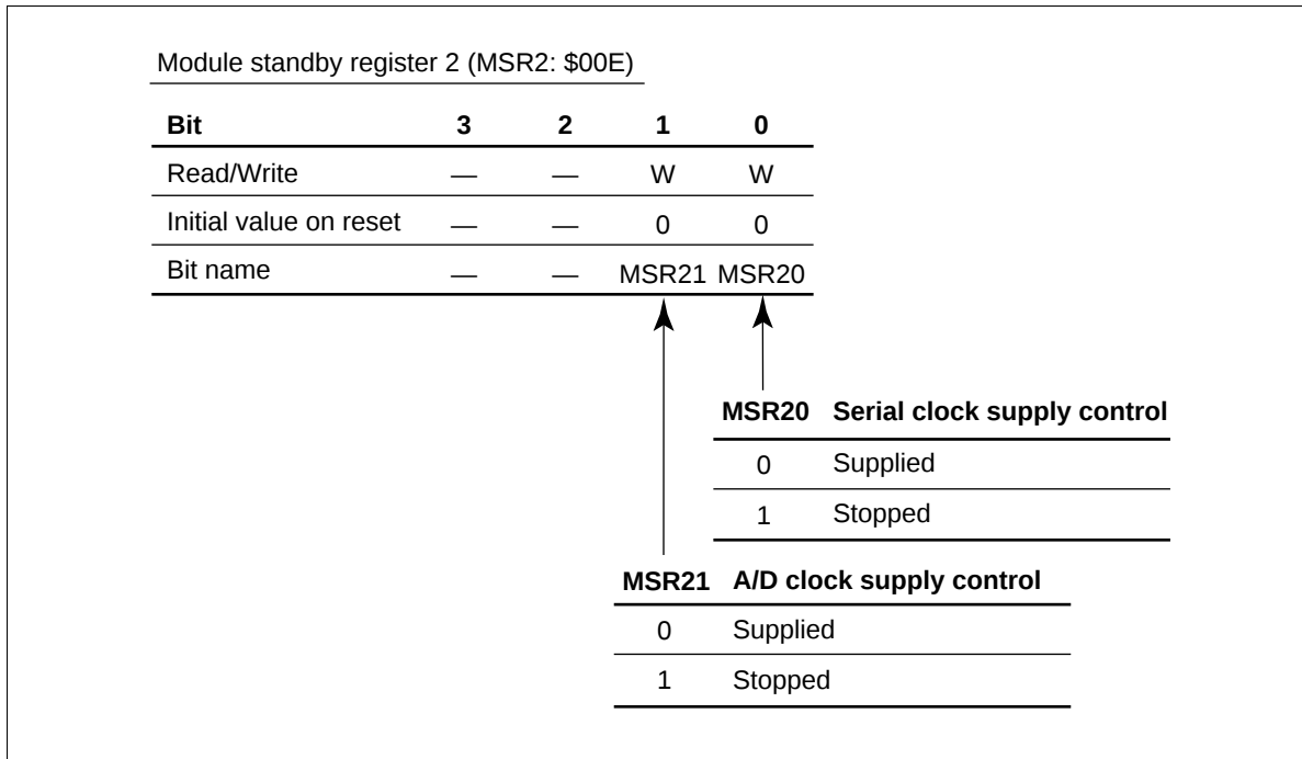
Figure 62 Module Standby Register 2 (MSR2)
