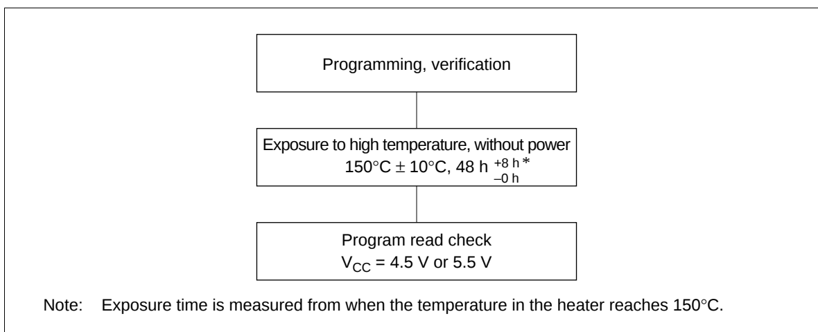
Figure 74 Recommended Screening Procedure
