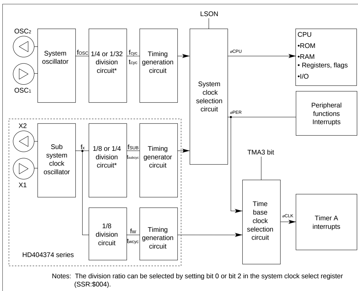
Figure 20 Clock Pulse Generator Circuit
