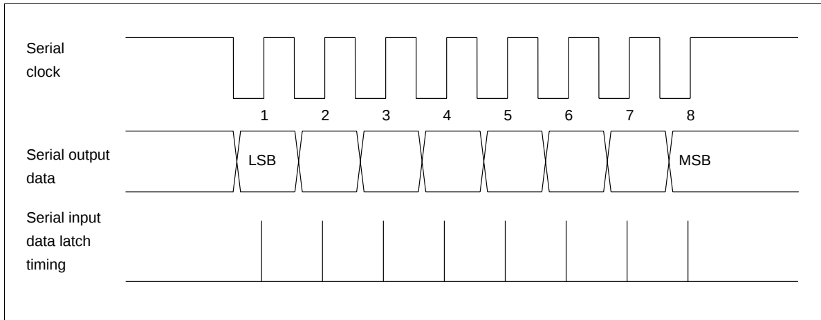
Figure 60 Serial Interface Input/Output Timing Chart
