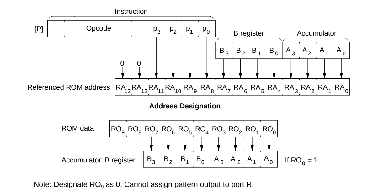
Figure 77 P Instruction
