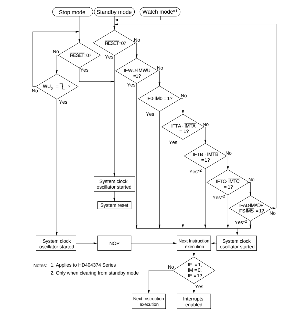
Figure 12 MCU Operation Flowchart
