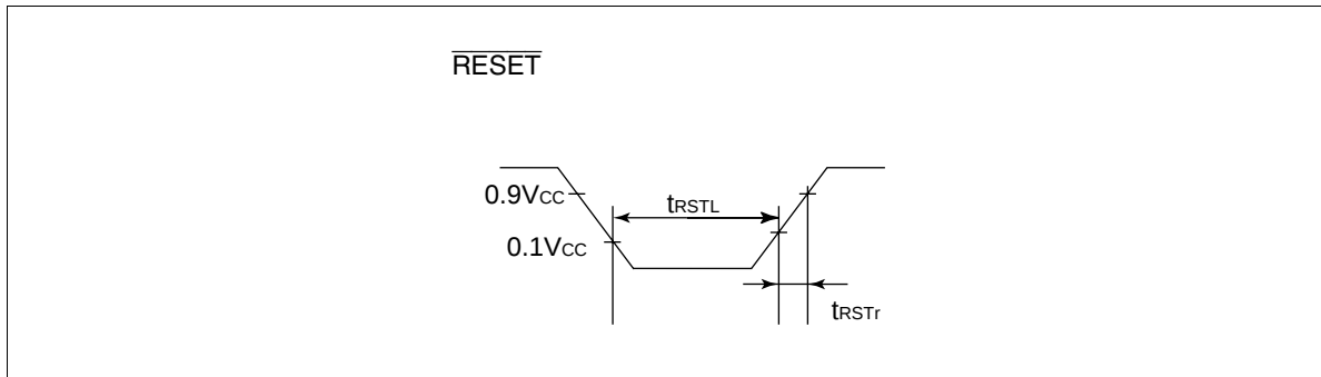
Figure 81 Reset Timing
