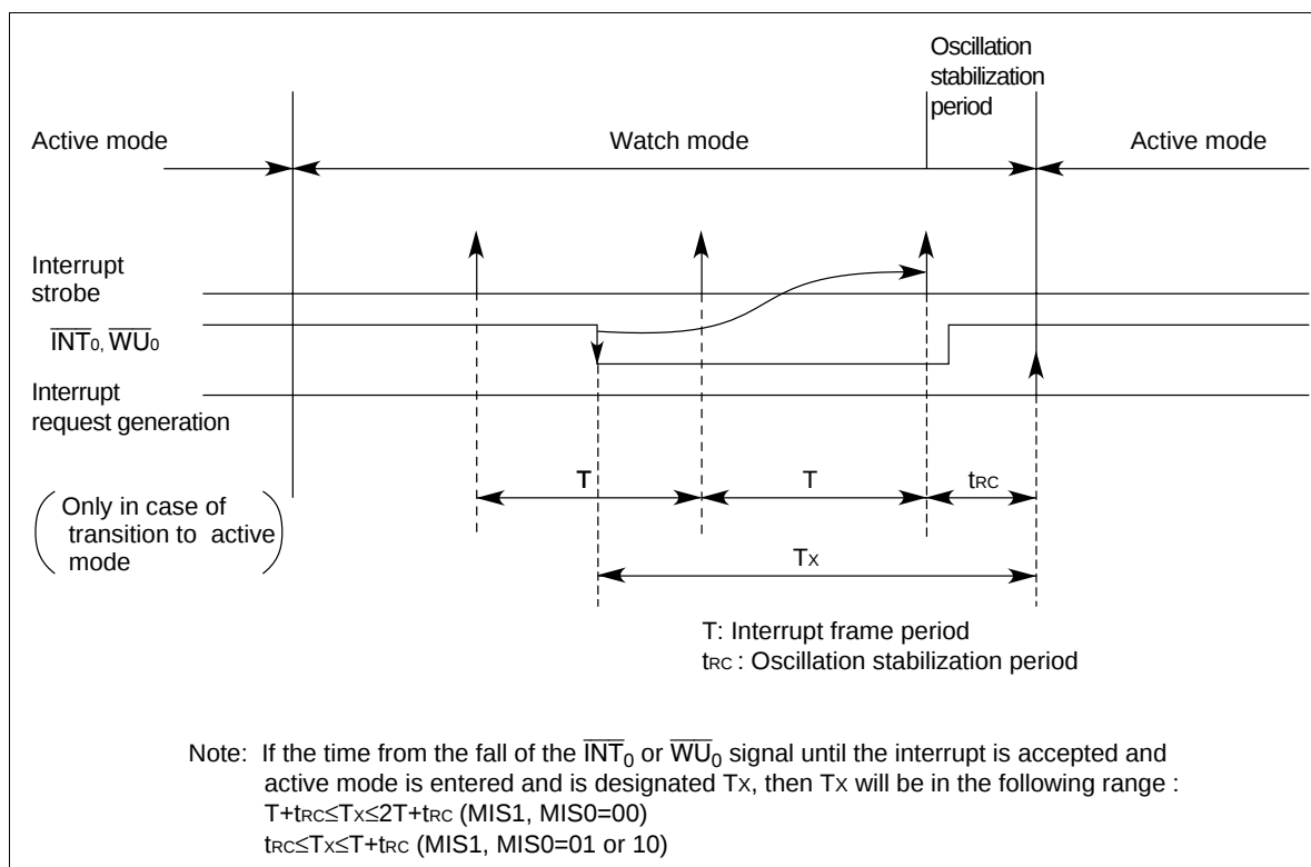
Figure 14 Interrupt Frame
