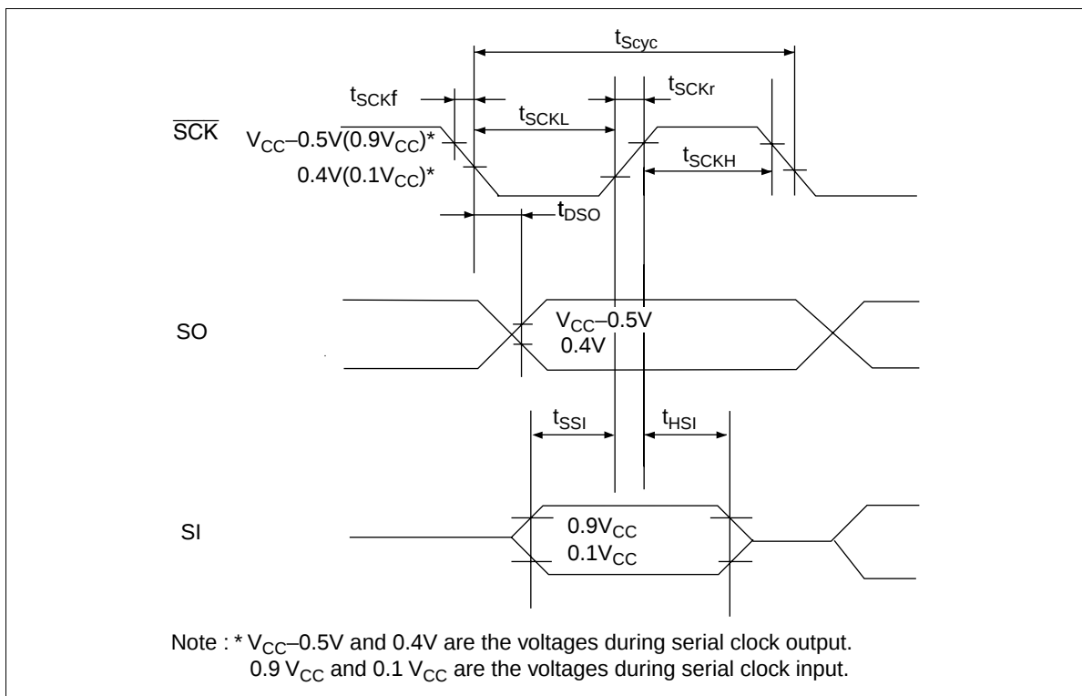
Figure 82 Serial Interface Timing
