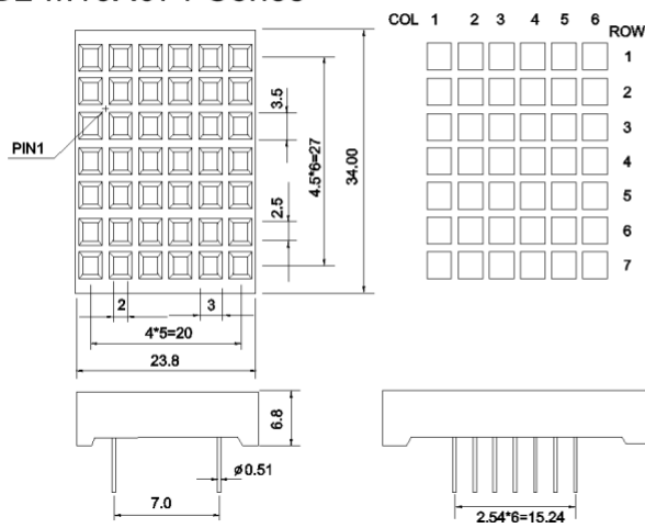
BL-M13X671 Series
