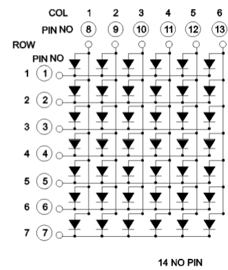
BL-M13B671
