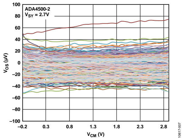
Figure 7. Input Offset Voltage ( V_{OS} ) vs. Common-Mode Voltage ( V_{CM} ), V_{SY} = 2.7\text{V}
