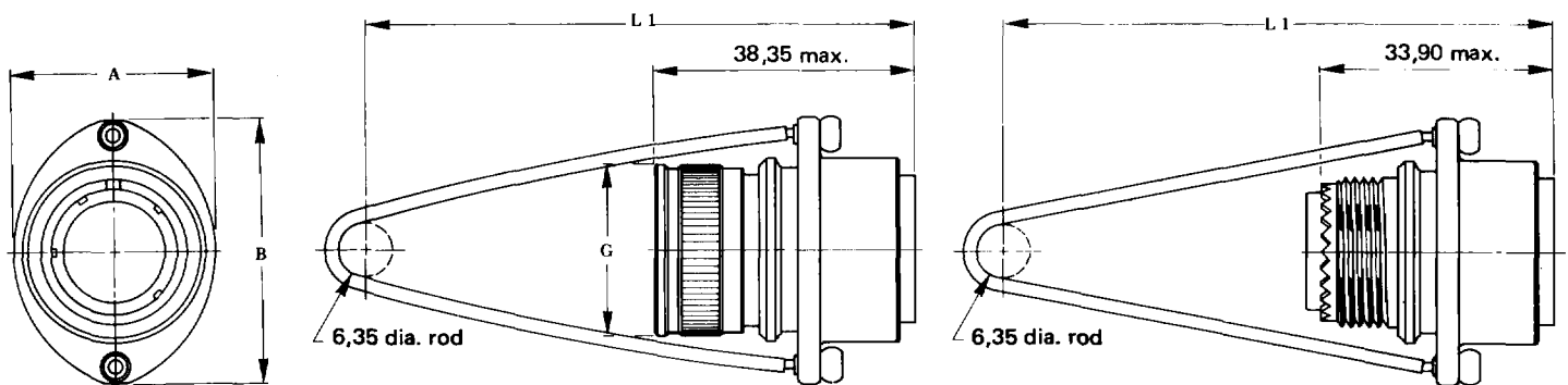
WITH BACKSHELL
