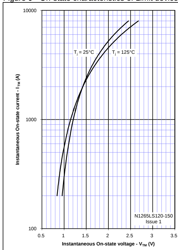
Figure 9 - On-state characteristics of Limit device
