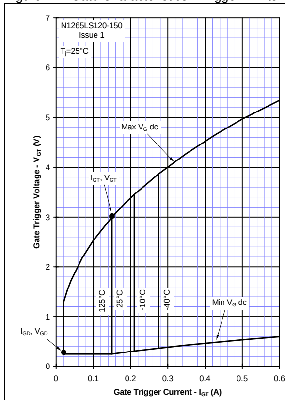
Figure 11 - Gate Characteristics - Trigger Limits
