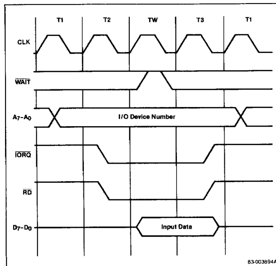
Figure 6. I/O Read Cycle
