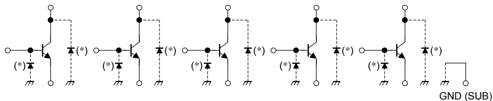
TD62507PG/FG
