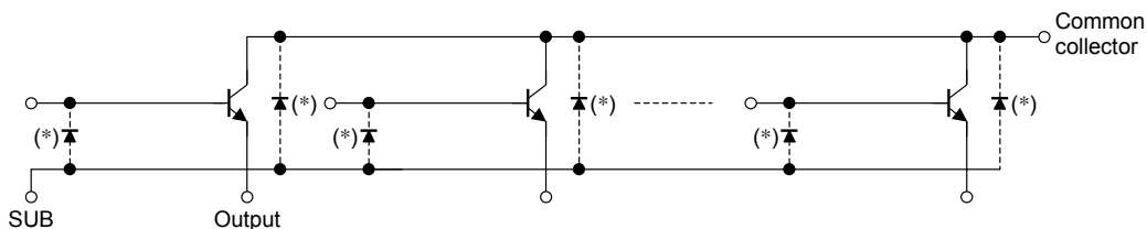
TD62505PG/FG
