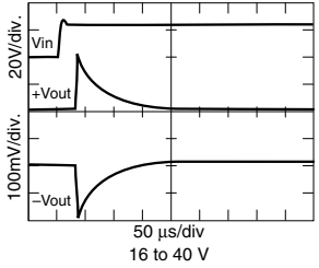
SMFL2815D Step Line Response
