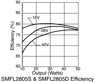
SMFL2805S & SMFL2805D Efficiency
