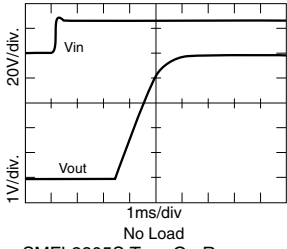
SMFL2805S Turn On Response
