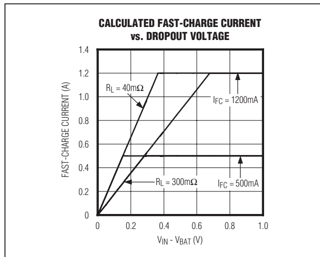
Figure 13. Calculated Fast-Charge Current vs. Dropout Voltage
