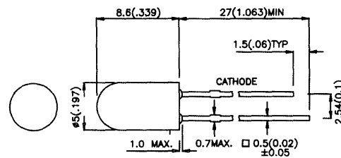
T-1 3/4 (5mm) Round
