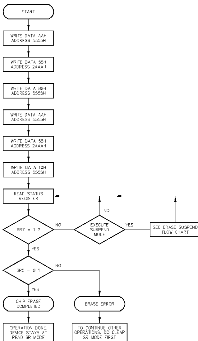
FIGURE 2: AUTOMATIC CHIP ERASE FLOW CHART
