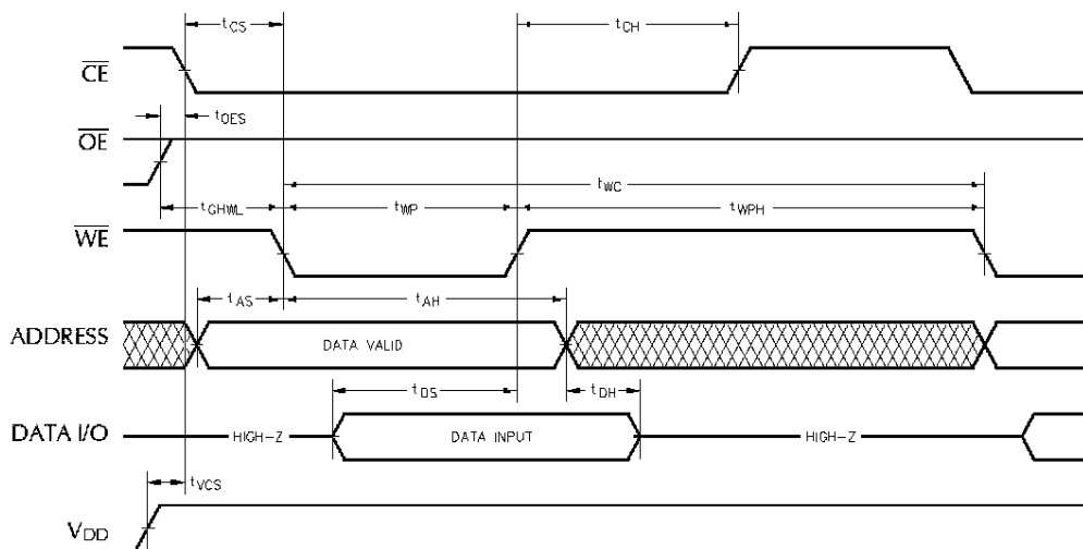
Figure 6: WRITE CYCLE
