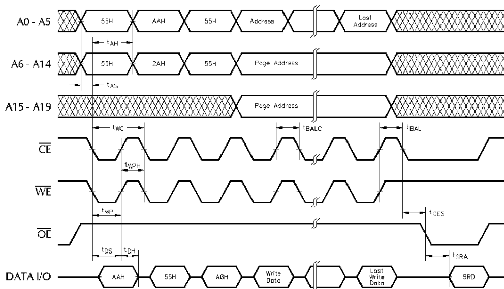
Figure 7: AUTOMATIC PAGE PROGRAM CYCLE 10
