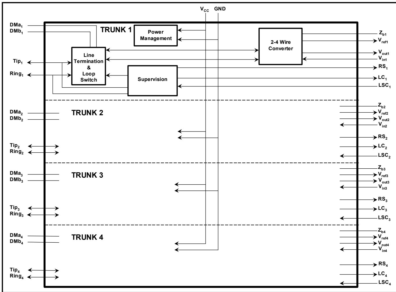
Figure 2: Block Diagram
