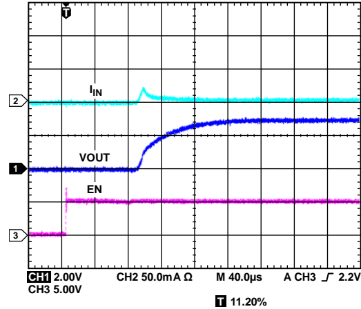
Figure 30. LDO Startup, V_{OUT3} = 3.0\text{ V} , I_{OUT3} = 5\text{ mA}
