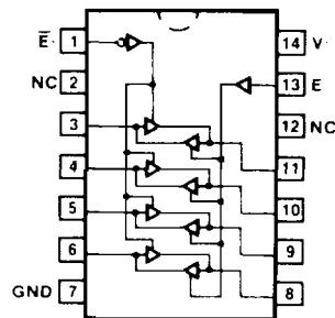
Pin Assignment for DIP and SOIC
