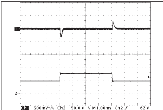
Figure 17: Output voltage response to step-change in input voltage ( 48\text{V} to 75\text{V} ), at 3.3\text{A} load current. Load cap: 15\ \mu\text{F} tantalum capacitor and 1\ \mu\text{F} ceramic cap. Ch1: V_{out} ( 500\text{mV}/\text{div} ), Ch2: V_{in} ( 50\text{V}/\text{div} )
