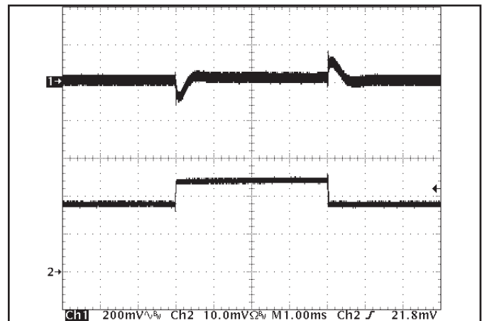
Figure 12: Output voltage response to step-change in load current (50%-75%-50% of I out (max); di/dt=1A/µs). Load cap: 470µF electrolytic, 15µF tantalum and 1µF ceramic cap. Ch 1: V out (200mV/div), Ch 2: I out (1A/div).
