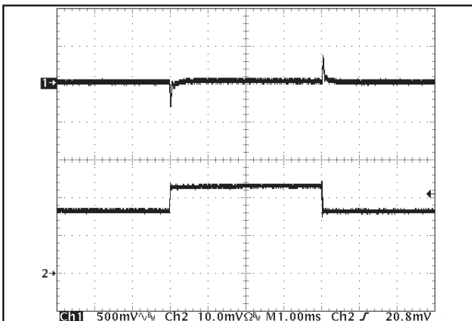
Figure 11: Output voltage response to step-change in load current (50%-75%-50% of I out (max); di/dt=0.1A/µs). Load cap: 15µF tantalum cap and 1µF ceramic cap. Ch 1: V out (500mV/div), Ch 2: I out (1A/div).
