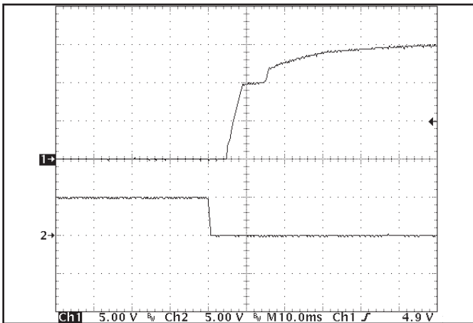
Figure 9: Turn-on transient at full load (resistive load) (10ms/div). Load cap: 15µF tantalum capacitor and 1µF ceramic cap. Input voltage pre-applied. Ch 1: V out (5V/div), Ch 2: ON/OFF input (5V/div).
