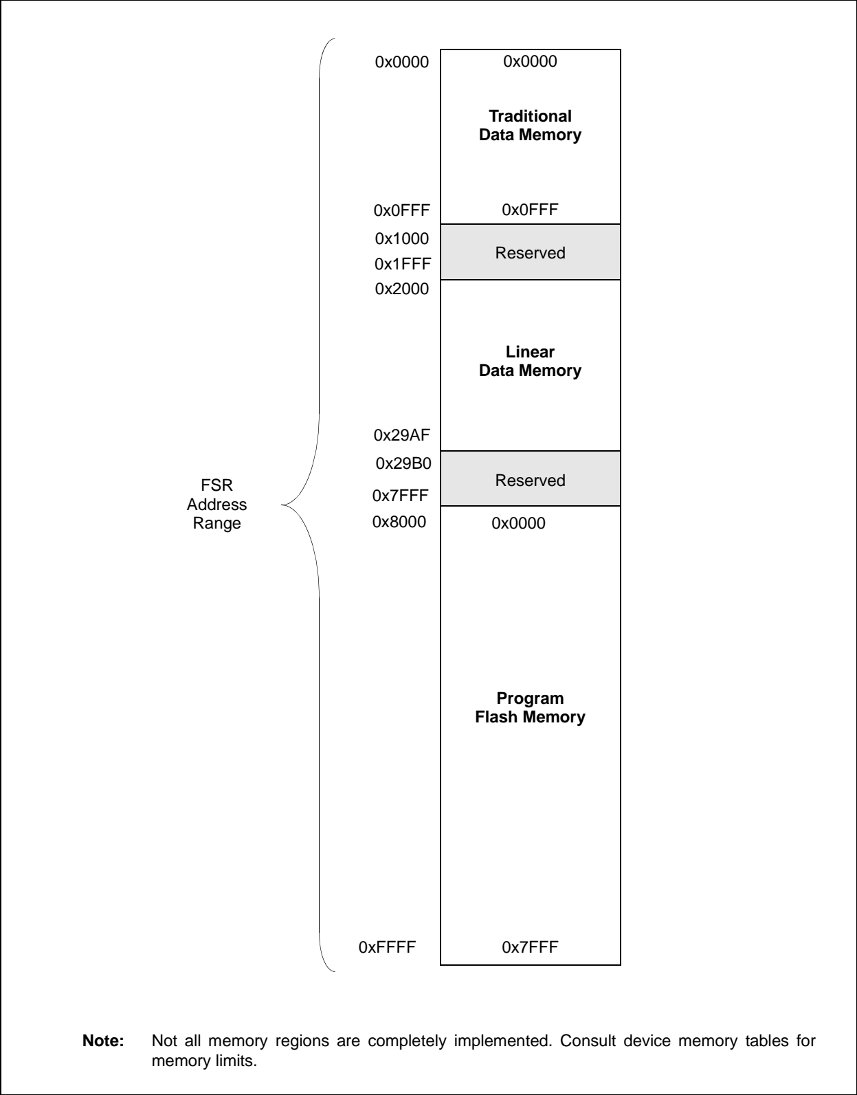
FIGURE 2-5: INDIRECT ADDRESSING
