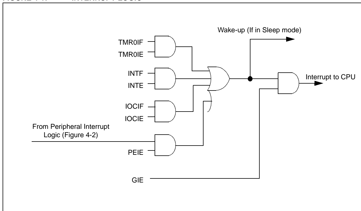
FIGURE 4-1: INTERRUPT LOGIC
