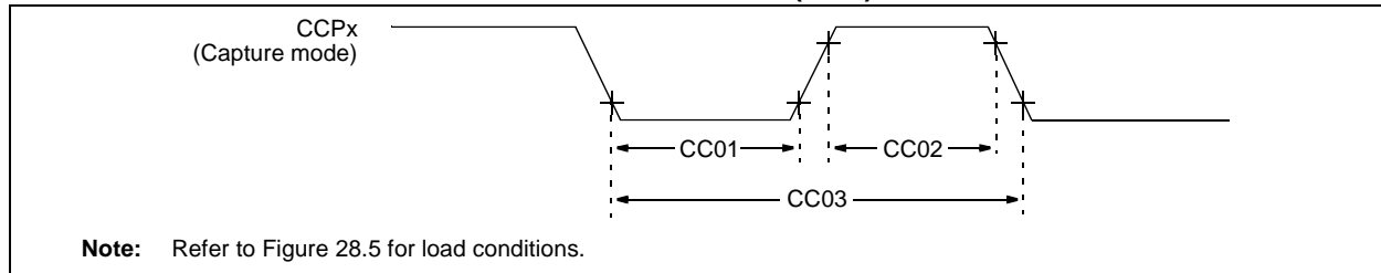
FIGURE 28-11: CAPTURE/COMPARE/PWM TIMINGS (CCP)
