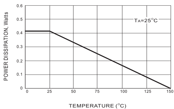
Fig.1 STEADY STATE POWER DERATING
