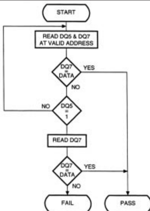
Figure 11 : Data Polling Flow-chart
