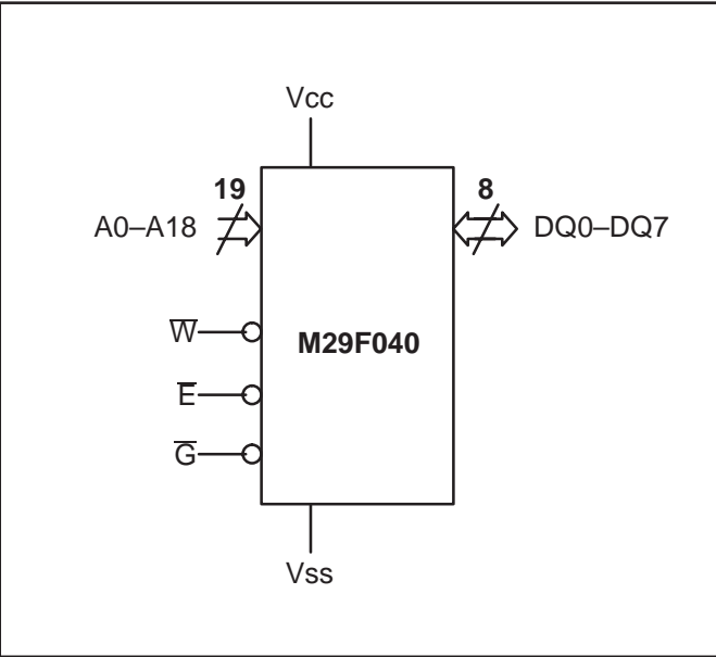
Figure 1 : Logic Diagram
