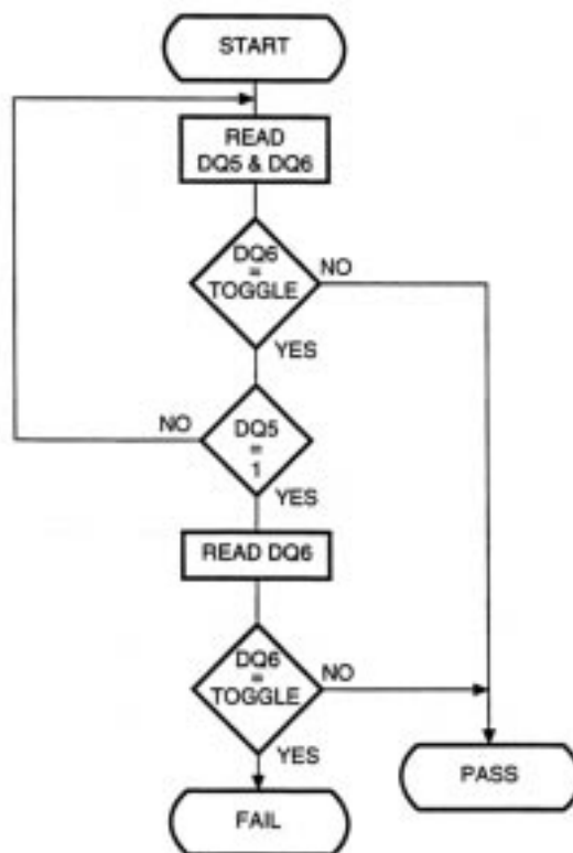
Figure 13 : Data Toggle Flow-chart
