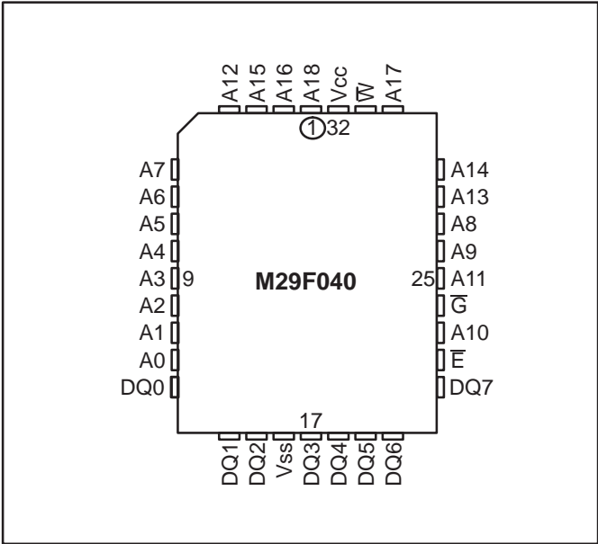
Figure 3 : PLCC and LCCC Pin Connections
