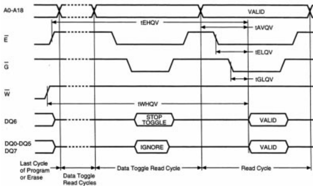
Figure 14 : Data Toggling DQ6 AC Waveforms
