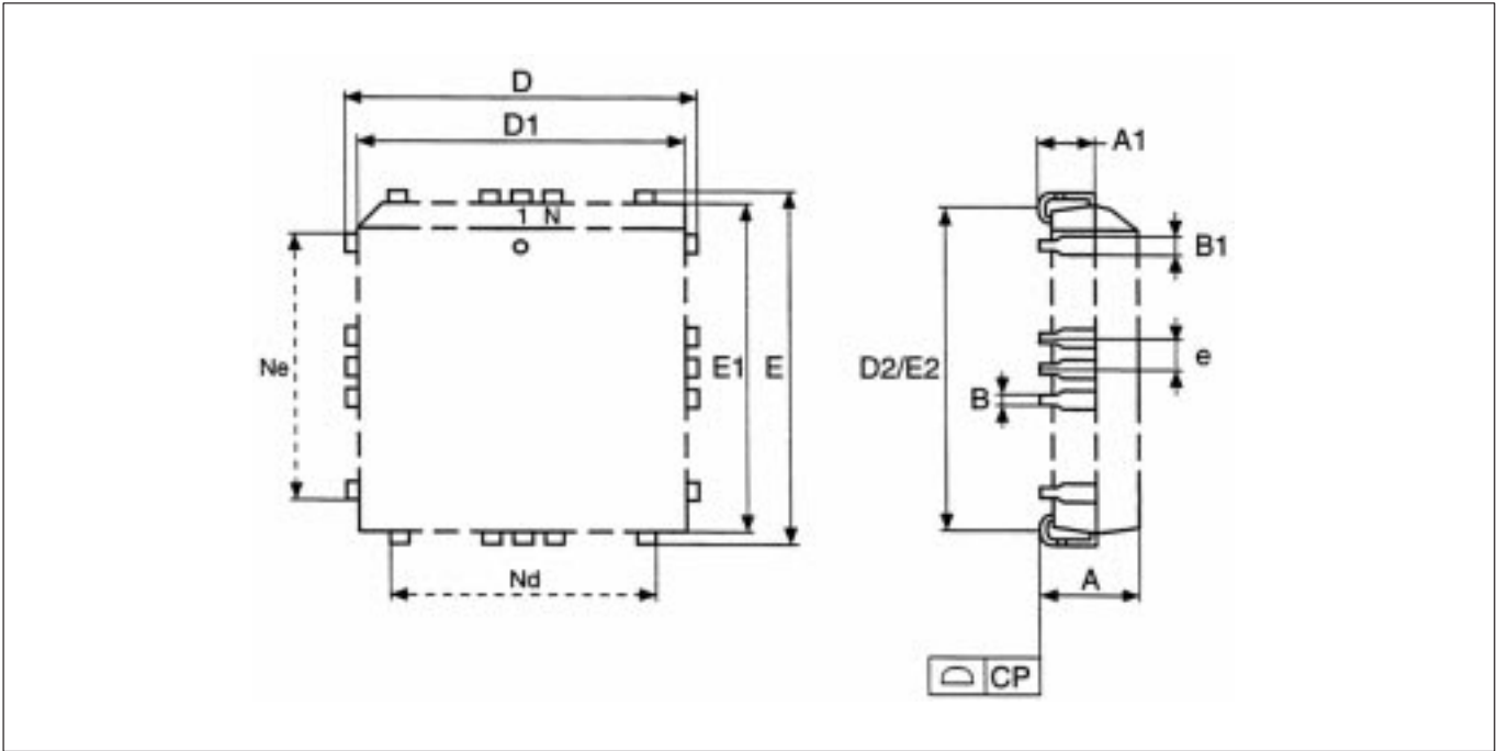
Drawing is out of scale
