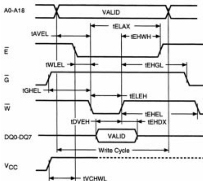
Figure 10 : Write AC Waveforms, \overline{E} Controlled
