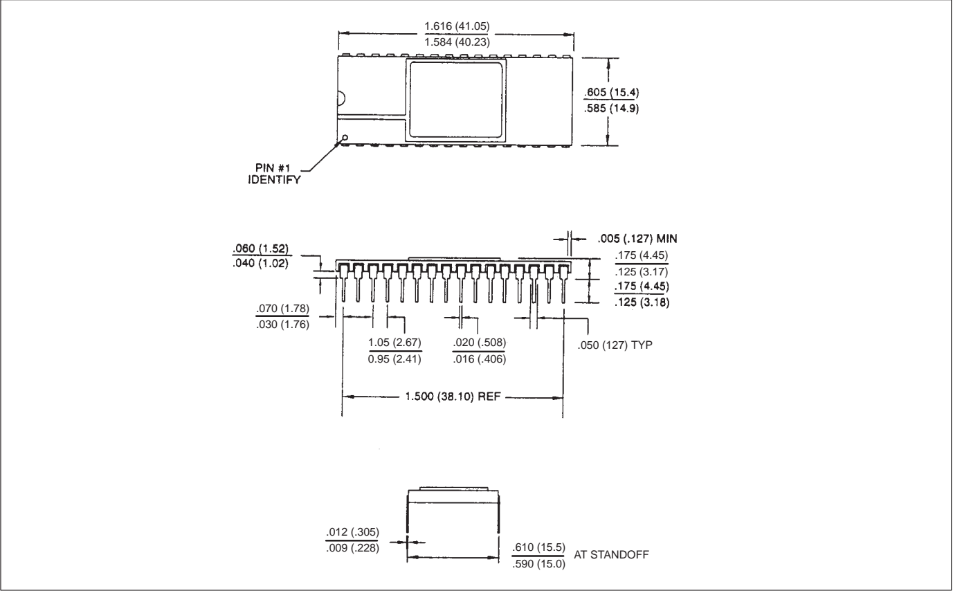
Drawing is out of scale
