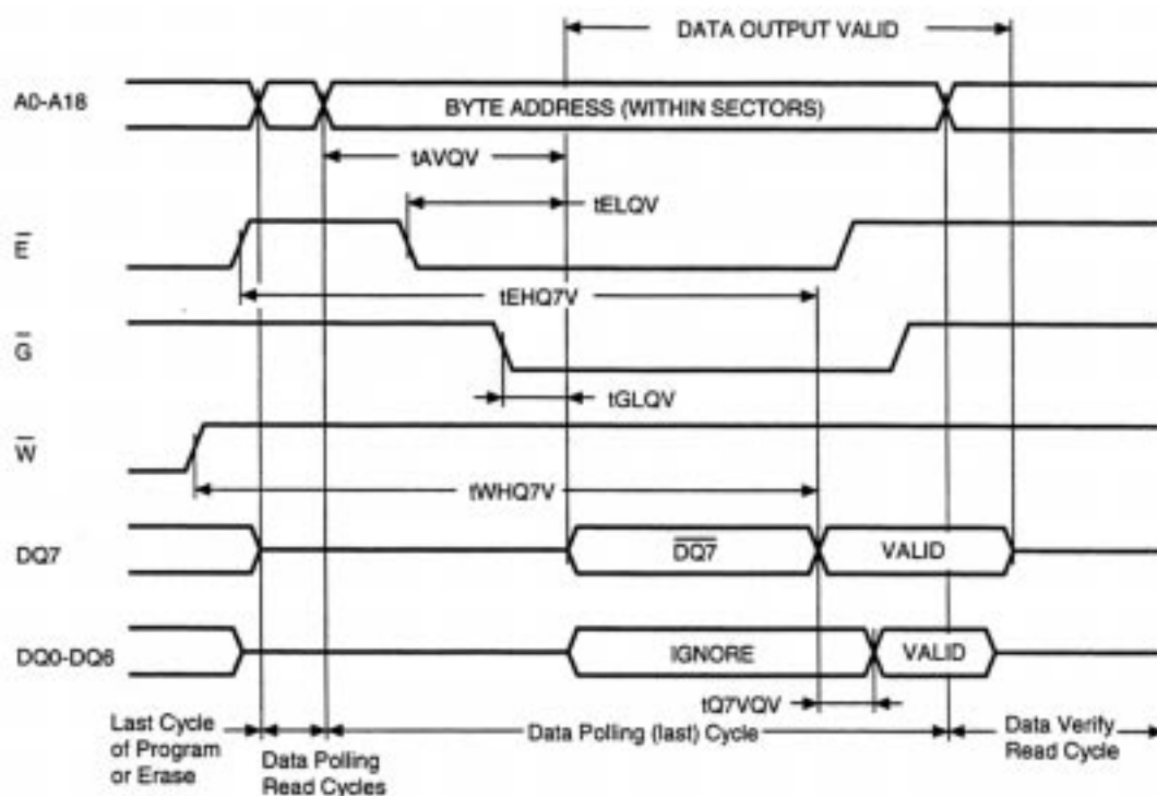
Figure 12 : Data Polling DQ7 AC Waveforms
