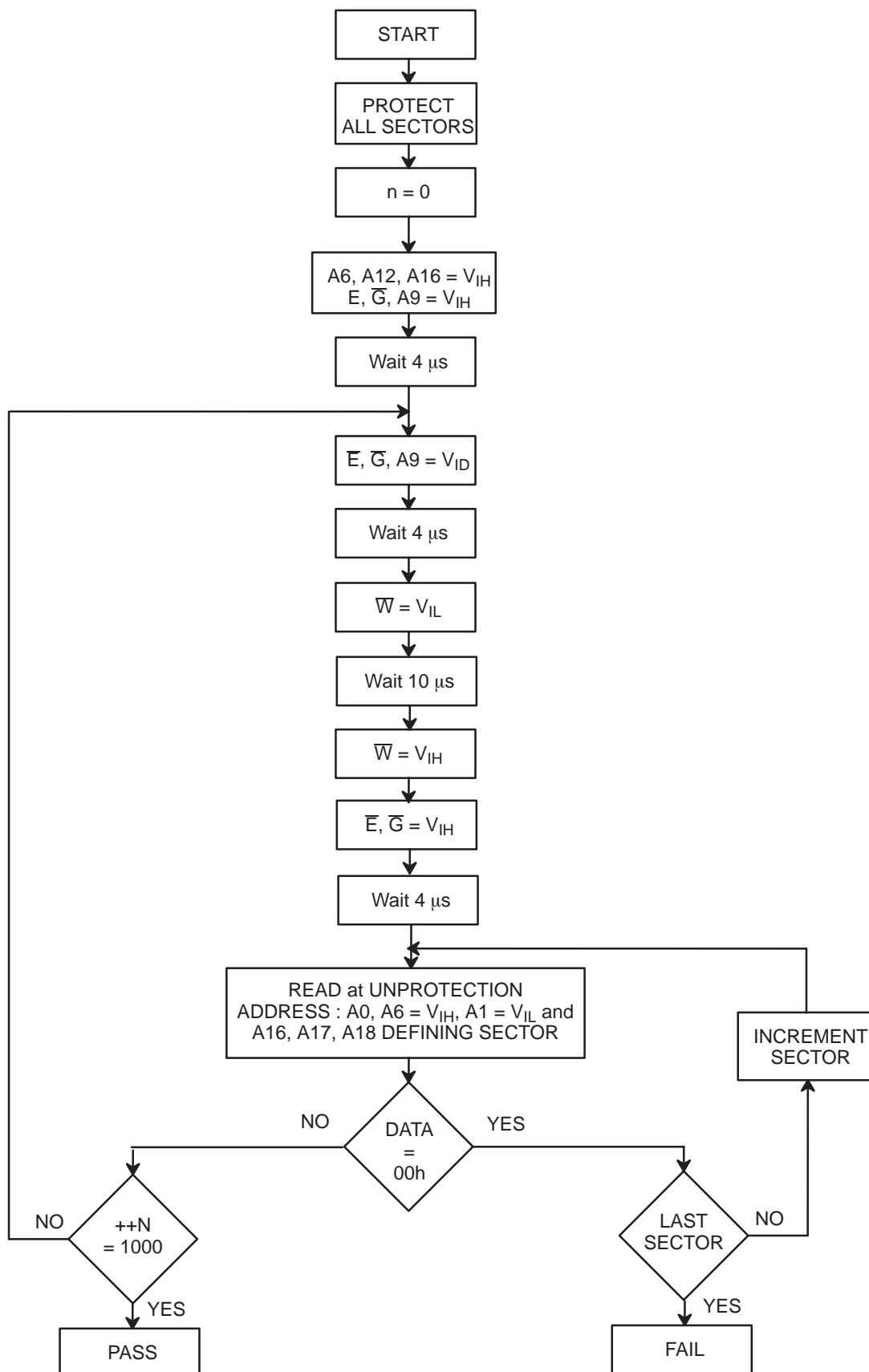
Figure 16 : Sector Unprotecting Flow-chart
