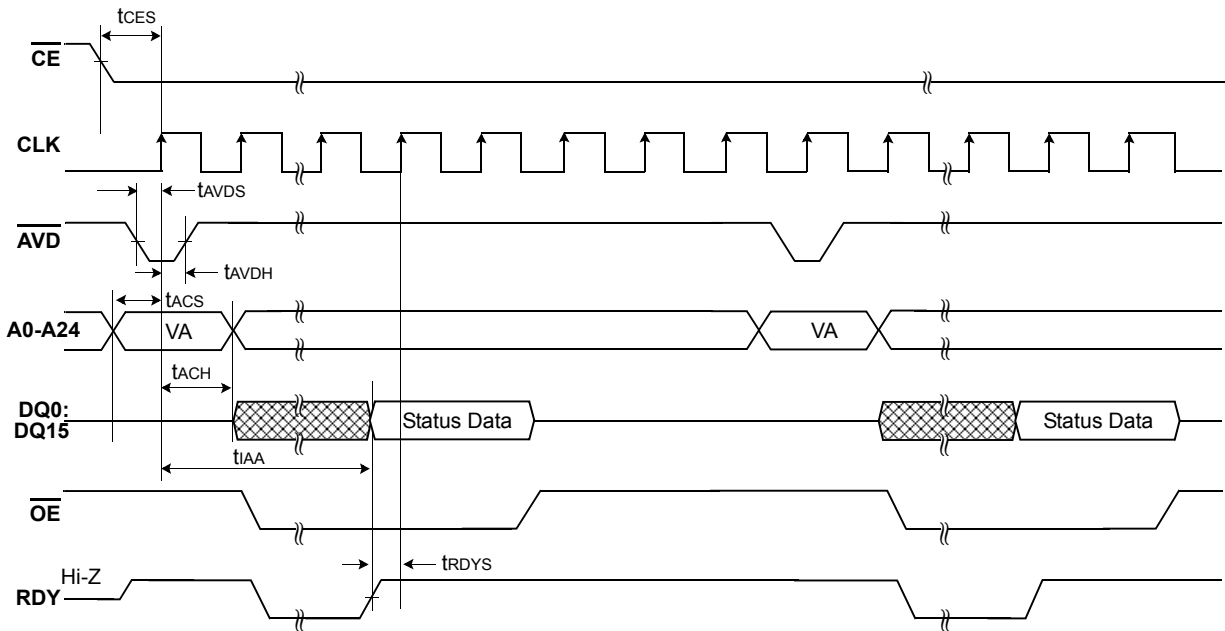
Figure 16. FLASH \overline{Data} Polling Timings (During Internal Routine)
