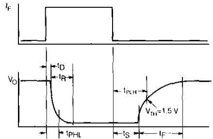
Figure 8. Switching waveforms
