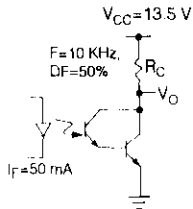
Figure 9. Switching schematic
