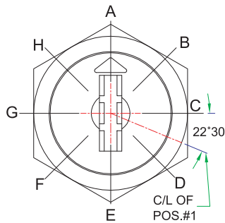
45° INDEXING
