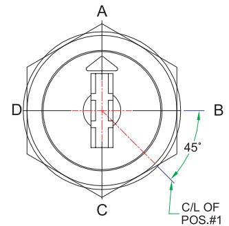
90° INDEXING
