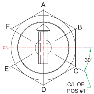
60° INDEXING
