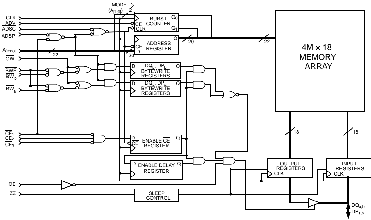
CY7C1482V33-4M x 18
