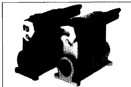
Surface mount base with side entry on the right, single locking lever and cover, high profile
